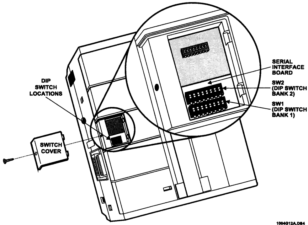
Figure 1. Okidata MicroLine 184 DIP Switch Location
